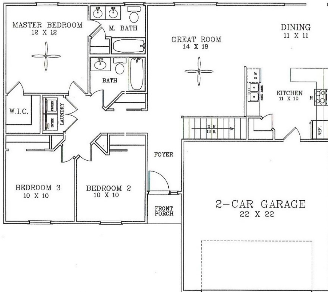
THE "RIVERSIDE" FLOOR PLAN 1255 SQ. FT.
